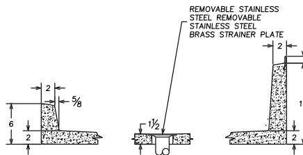
SECTION THRU THRESHOLD
