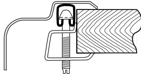
U-Channel Type Mounting System
